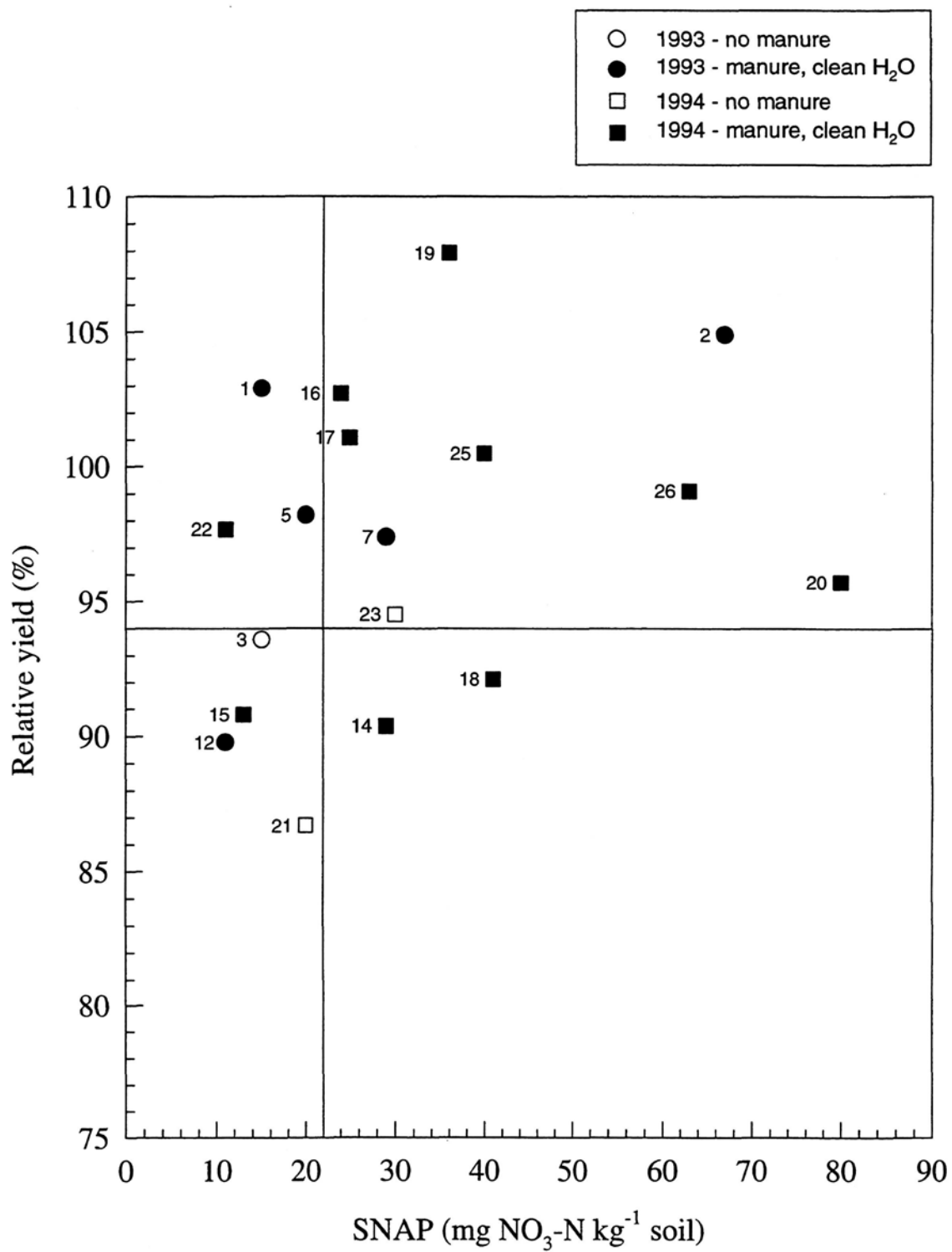
Fig. 4. Cate-Nelson plot of relative yield vs. soil nitrate at planting (SNAP). Numbers are site numbers.
