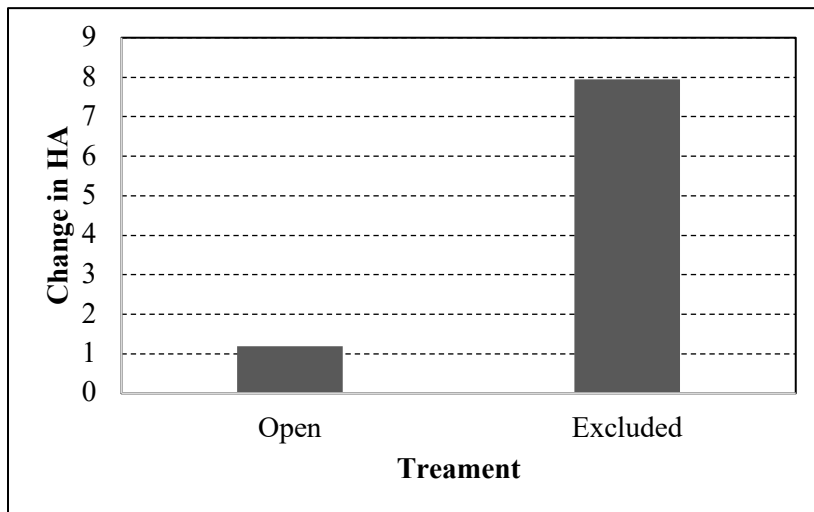
Figure 15: The effect of natural enemy exclusion on hops aphid in Starksboro, VT in August.
