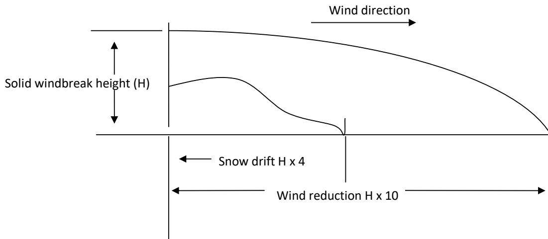
Figure 1. Typical wind and snow patterns resulting from windbreak placement. Adapted (Harner et al., 2011).
