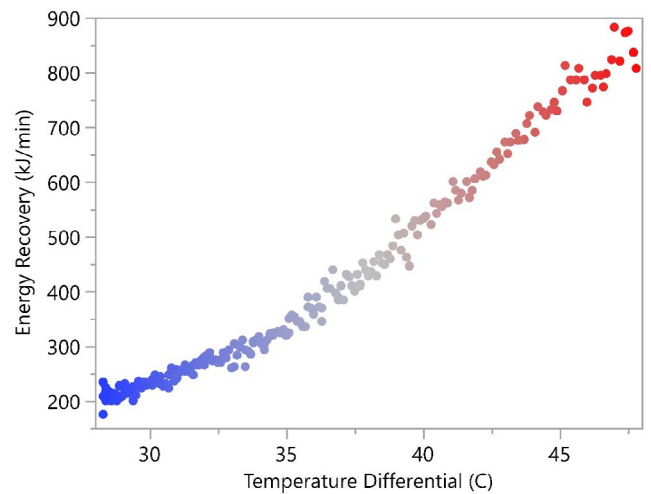
Fig. 5. Energy gain vs. temperature differential. Energy gain measured by increases in temperature in the heat sink tank (HST) as a function of the difference in temperatures between the vapor stream and the water in the HST.
