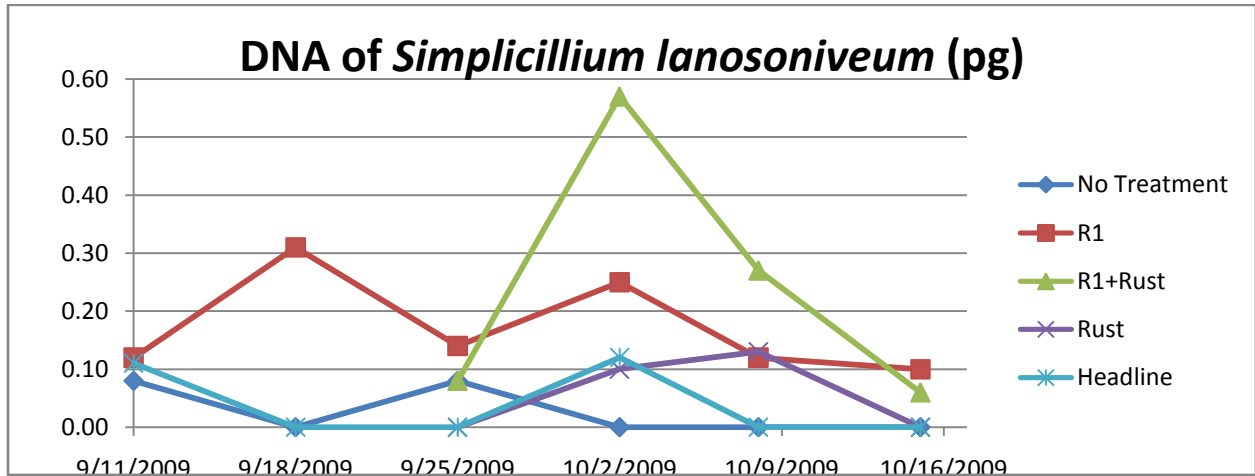
Figure 1. Quantitative measurements of DNA of (A) Simplicillium lanosoniveum and (B) Phakopsora pachyrhizi as determined by realtime PCR (q-PCR). Figure reflects measurements taken between pod formation (R4) and physiological maturity.
