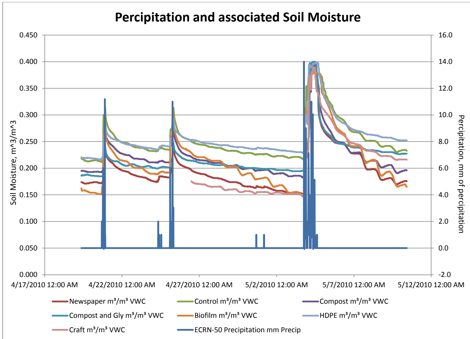
Figure 10. Precipitation and associated soil moisture under each mulch as measured in the top vertical six inches of soil.
