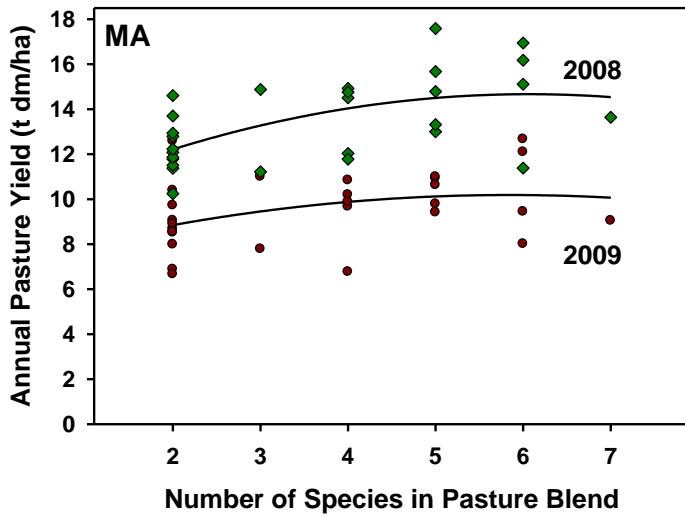
Figure 1. Total annual yields for blends in MA.
