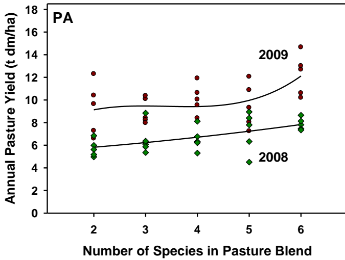
Figures 2. Total annual yields for blends in Pennsylvania.
