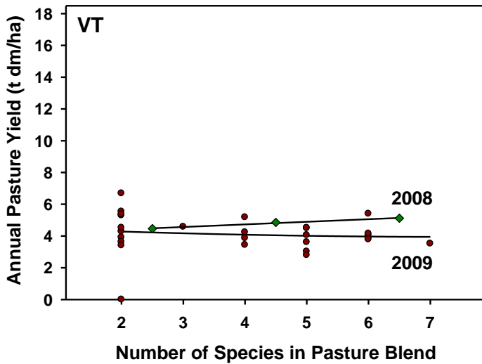
Figures 3. Total annual yields for blends in Vermont.
