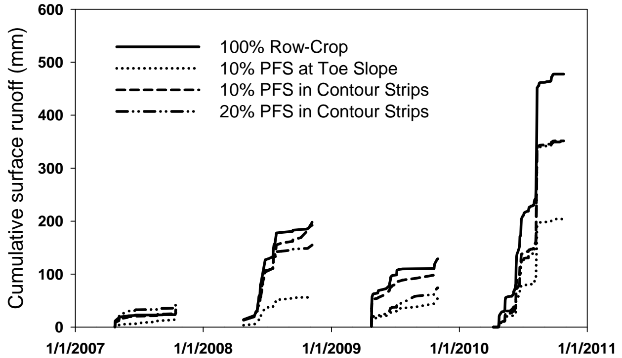
Figure 1: Surface runoff in 2007, 2008, 2009, and 2010 (PFS – prairie filter strips)
