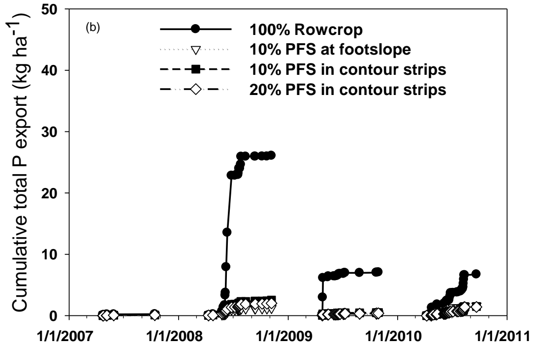
Figure 3: Impact of perennial filter strips on cumulative (a) total N and (b) total P in surface runoff.
