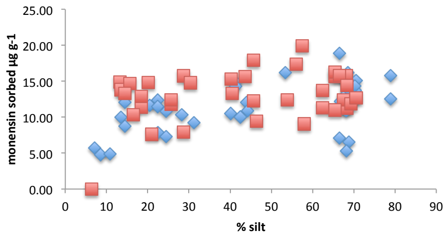
Sorption of monensin vs. % silt
