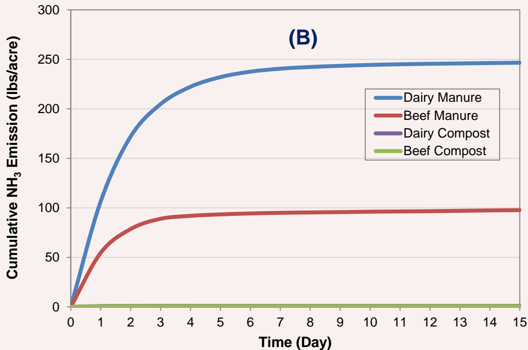
Figure 3. (A) Daily and (B) Cumulative NH 3 Emissions from Different Types of Manure Source
