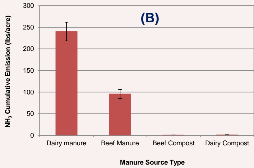
Figure 5. Summary of (A) CO 2 , (B) NH 3 , (C) CH 4 Emissions from Different Types of Manure Source
