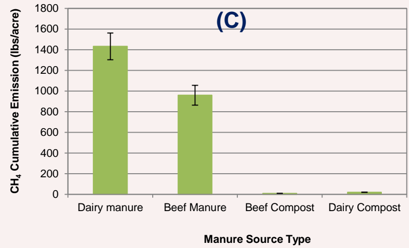
Figure 5. Summary of (A) CO 2 , (B) NH 3 , (C) CH 4 Emissions from Different Types of Manure Source
