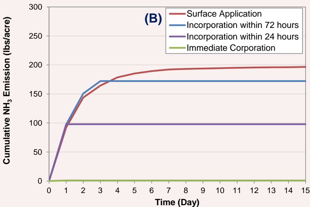
Figure 7. (A) Daily and (B) Cumulative \text{NH}_3 Emissions from Different Incorporation Times
