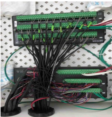
Sensors connected to data logger
