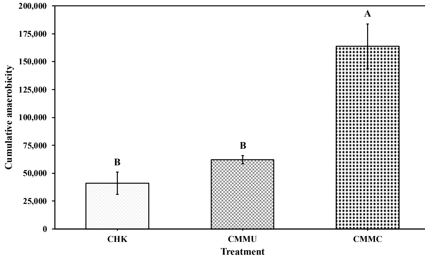
Figure: Effect of anaerobic soil disinfestation (ASD) carbon source: nonamended check (CHK), and chicken manure, molasses without polyethylene plastic mulch (CMMU), and chicken manure, molasses with polyethylene mulch (CMMC) on cumulative anaerobicity (soil anaerobic condition) in greenhouse experiments in Charleston, SC.
