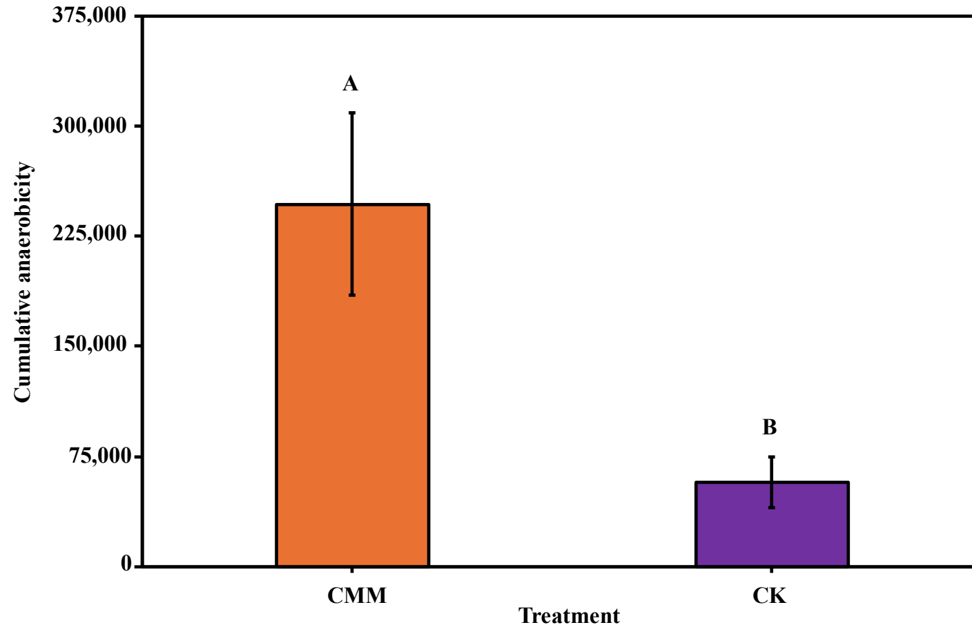
Figure: Impact of chicken manure and molasses (CMM)-induced anaerobic soil disinfestation on cumulative anaerobicity in microcosms under high tunnel conditions.
