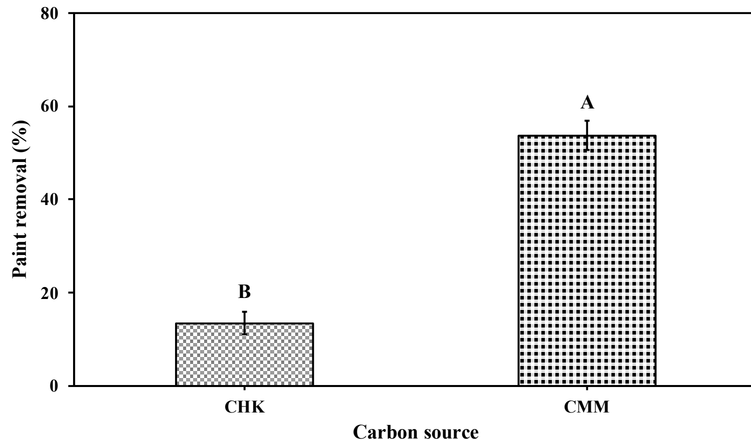
Figure: Effect of anaerobic soil disinfestation (ASD) carbon source: nonamended check (CHK), and chicken manure, molasses (CMM) on indicator of reduction in soil (IRIS) tubes at the time of ASD termination in field trials in Blackville, SC 2023-2024.
