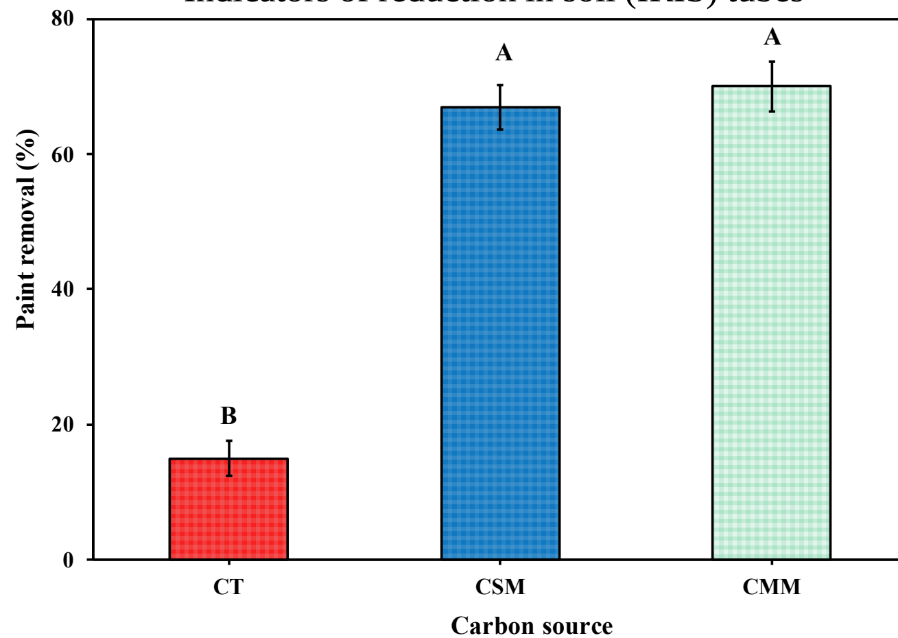
Figure: Effect of anaerobic soil disinfestation (ASD) carbon sources: nontreated control (CT), cottonseed meal (CSM), and chicken manure, molasses (CMM), on Indicators of Reduction in Soils (IRIS) tube paint removal (%) in field trials in Charleston, SC 2023-2024.
