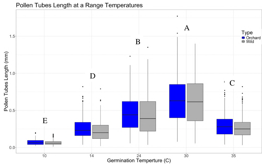
Figure 1. Pollen tube lengths over temperature from 10°C to 35°C. Populations of 100 tubes per pollen type per temperature are represented in standard box plots (boxes encompass values that fall within the 25 th and 75 th percentiles, the vertical line within the boxes indicate median values, whiskers denote range of values within the 10 th and 90 th percentiles, circles indicate values that are beyond the 10 th or the 90 th percentile).
