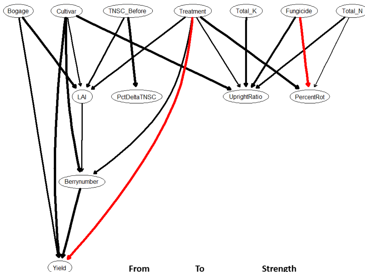
Figure 21: Edge strength of the conditional Gaussian Bayesian networks from structure learning: Strength Plot
