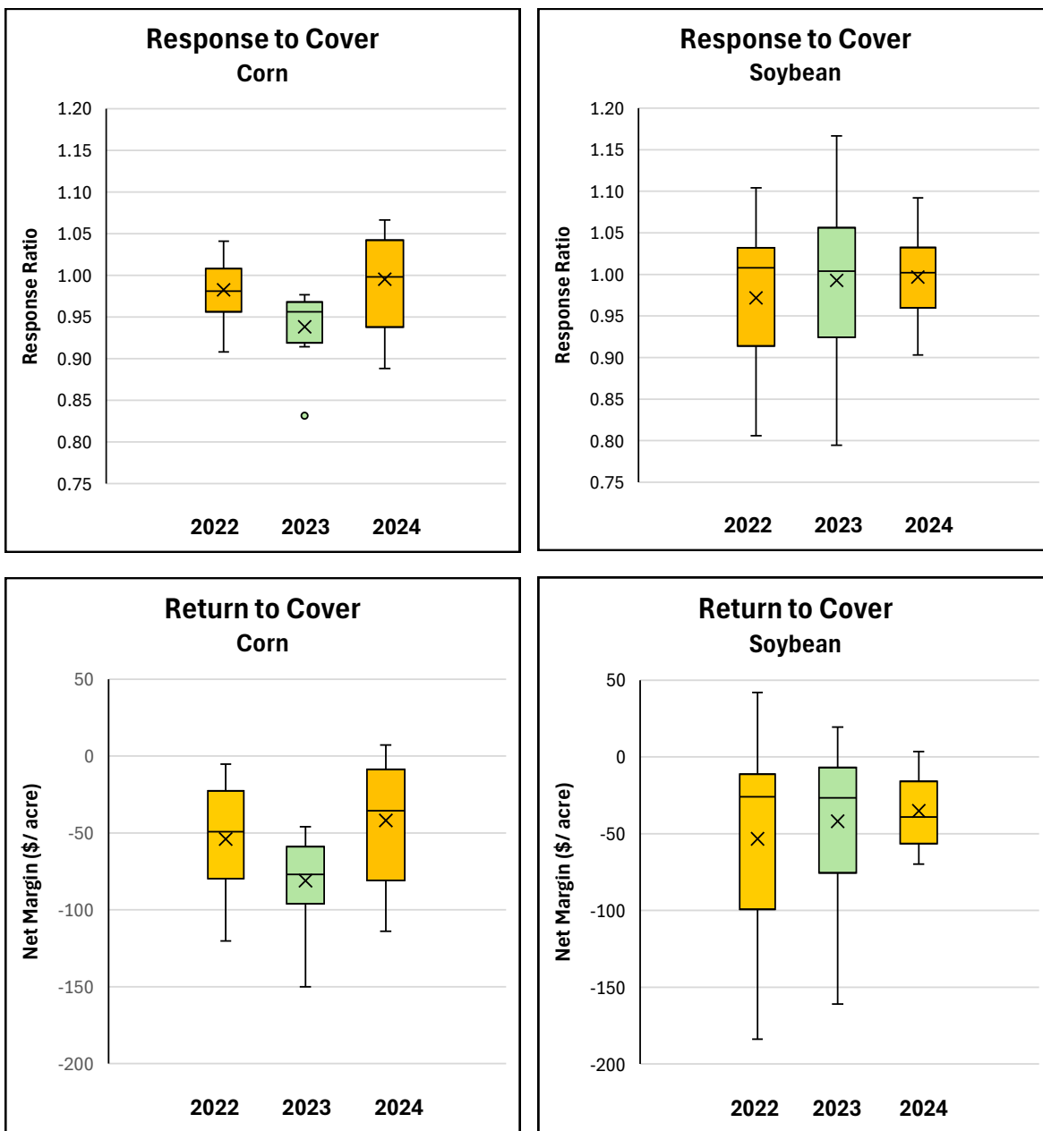
Figure 3. Annual yield response and net margin of corn and soybean following cereal rye.
