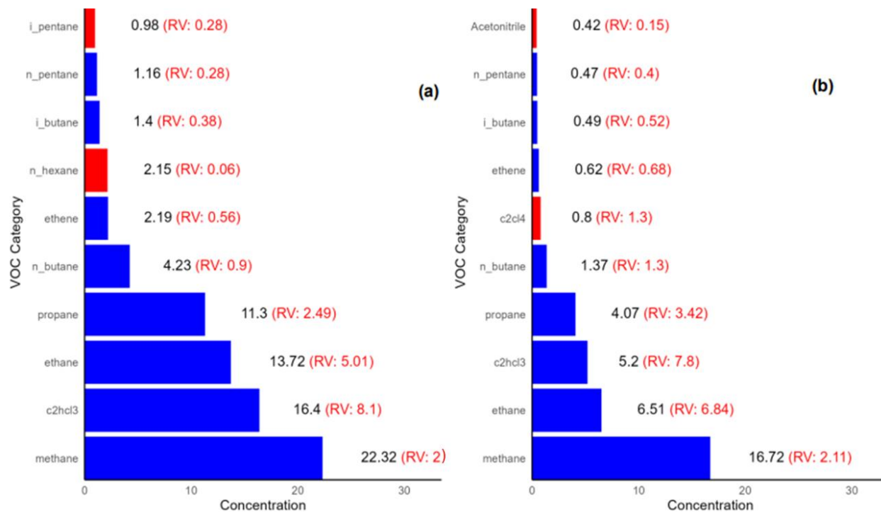
Figure 5. Top 10 volatile organic compounds (VOC) ranked by concentration (ppm) in the cow housing barns of Farm A and B. Values in red are reference air quality values measured in an open-air space in Colorado.
