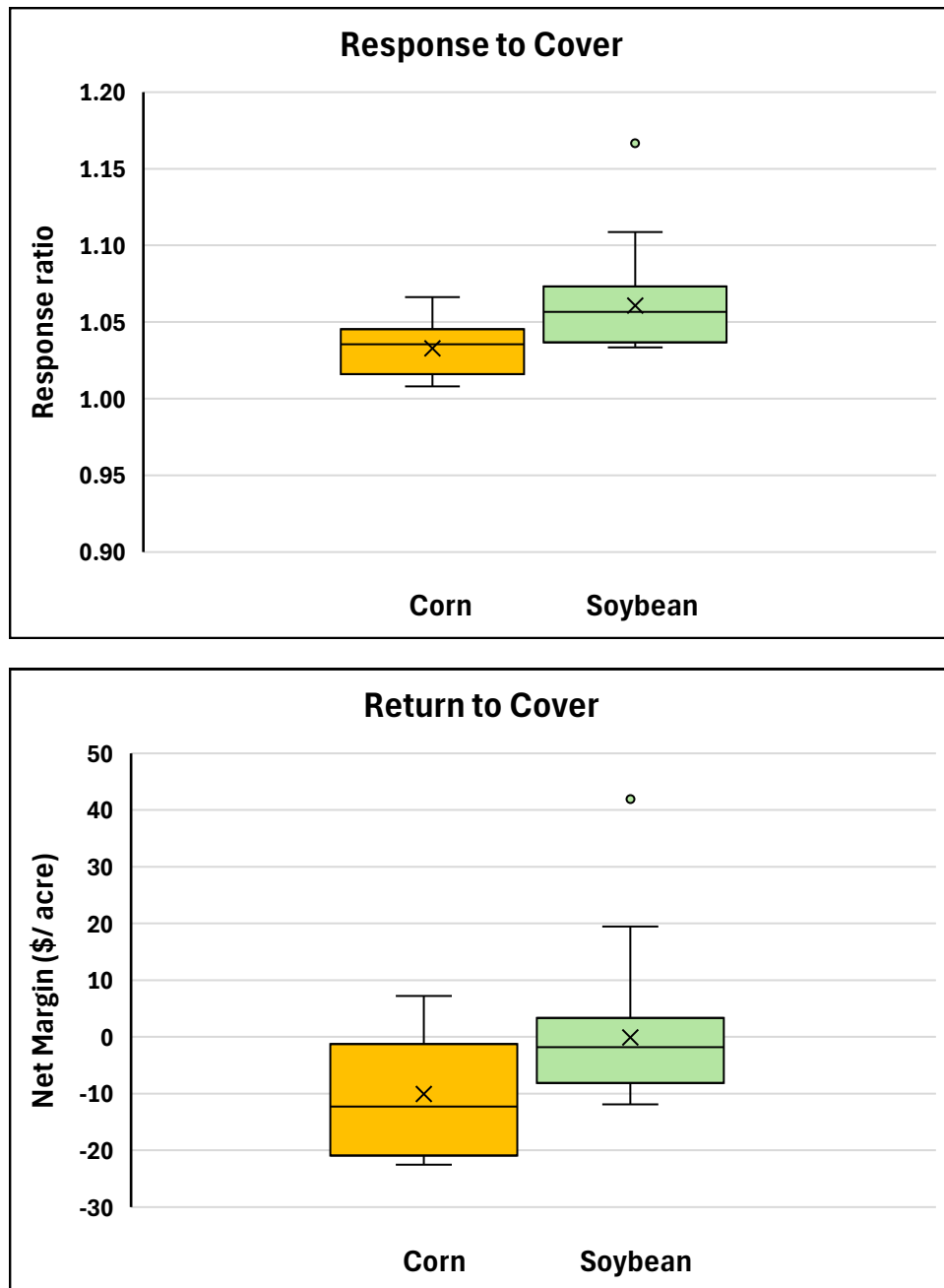
Figure 7. Yield response and net margin (return to cover) of corn and soybean following cereal rye, top 25% (upper quartile) of responses, 2022- 2024.
