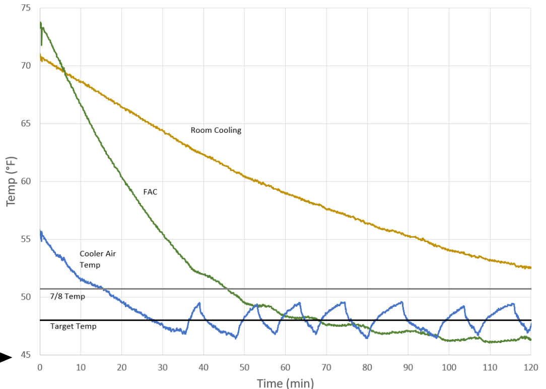
Figure - Comparison of roasting peppers cooled using room cooling and forced air cooling methods.
