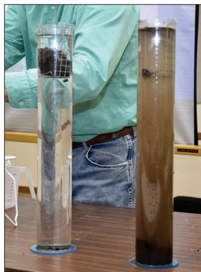
Photo: J. Johnson, Iowa NRCS This slake test shows that the soil on the right has poor aggregate stability, which could lead to reduced water infiltration and root penetration.
