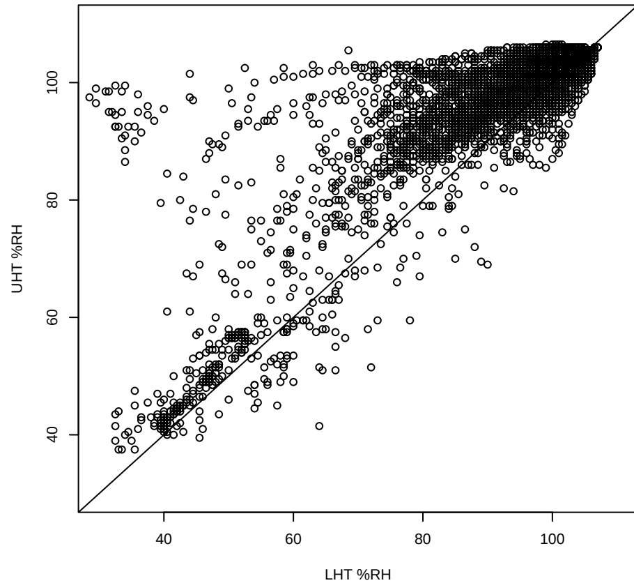
Comparing %RH in UHT vs. LHT to a 1:1 relationship
