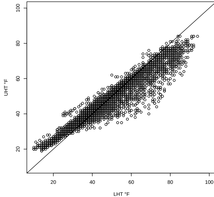
Comparing Temp in UHT vs. LHT to a 1:1 relationship
