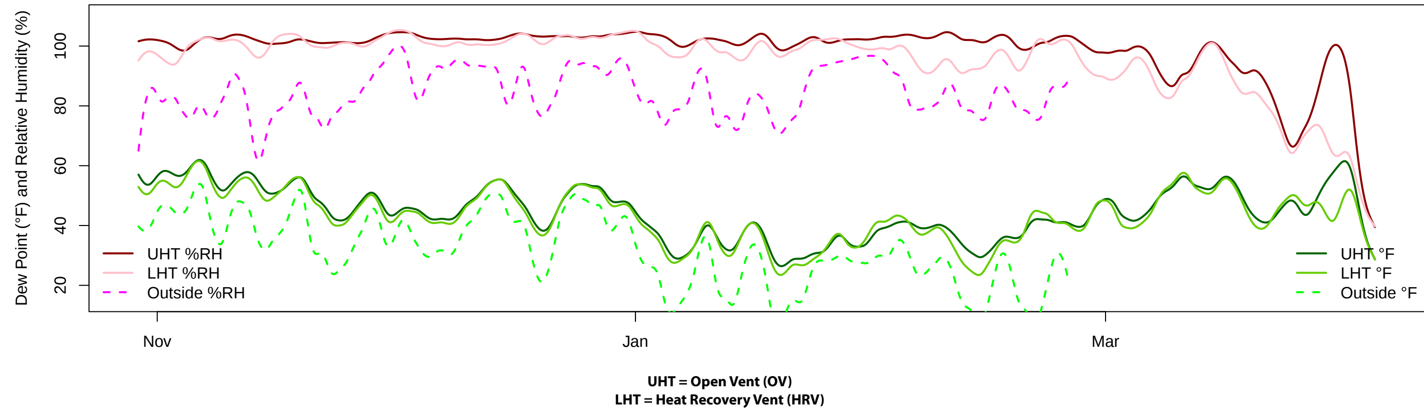
Dew Point and Humidity Across All Three Treatments (Smoothed)
