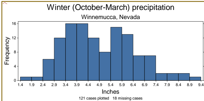
Figure 63 Histogram
