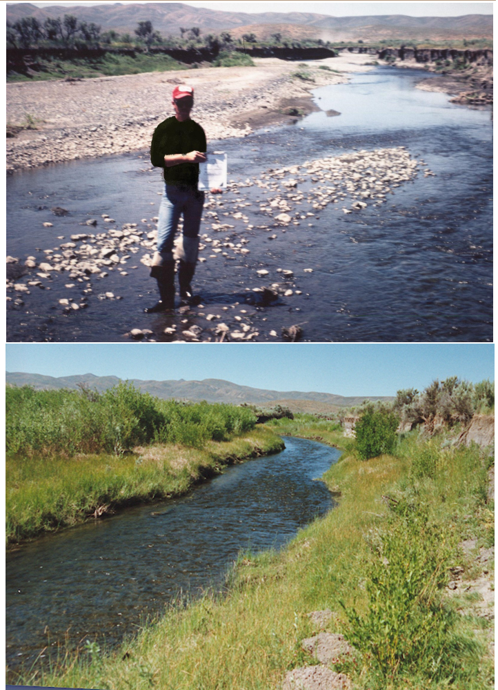
Figure 30. Many streams that do not meet water quality standards or that could meet water quality goals at a higher level have been impacted by loss of riparian functions. Regaining functions can recover water and aquatic habitat quality such as happened on Maggie Creek (Kozlowski et al. 2013).
