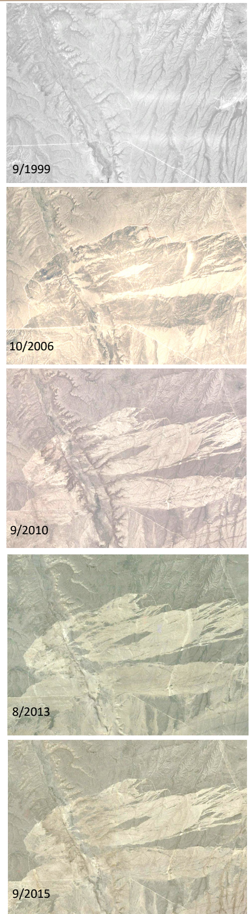
Figure 54. Images from google Earth of a Nevada 2006 fire.
