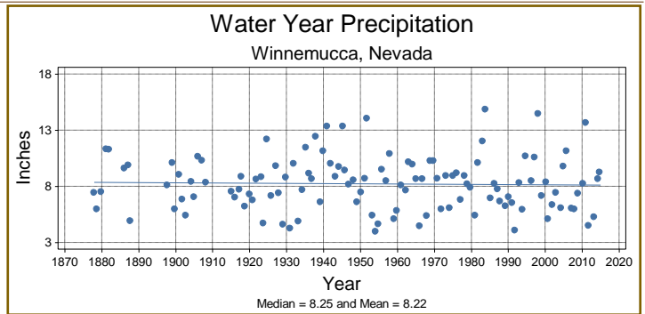
Figure 65 Scatter plot
