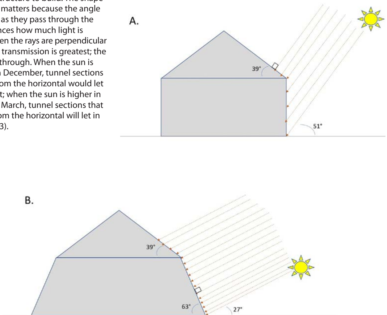
Figure 3. The angle of the sun above the horizon influences transmission of solar radiation through different parts of a high tunnel. Sections oriented 90^\circ to the rays of the sun will transmit the most radiation. A. Example at the Spring equinox in Indianapolis. The sun is 51^\circ above the horizon at its highest point. At that time an angled roof at 39^\circ from horizontal would be perpendicular ( 90^\circ , indicated by \square ) to the sun's rays and let in more radiation than the sidewalls. B. Example at the winter solstice in Indianapolis. The sun is 27^\circ above the horizon at its highest point. At that time an angled sidewall at 63^\circ from horizontal would be perpendicular to the sun's rays and let in more radiation than the angled roof or a straight sidewall. Sun angles obtained from www.esrl.noaa.gov/gmd/grad/solcalc/
