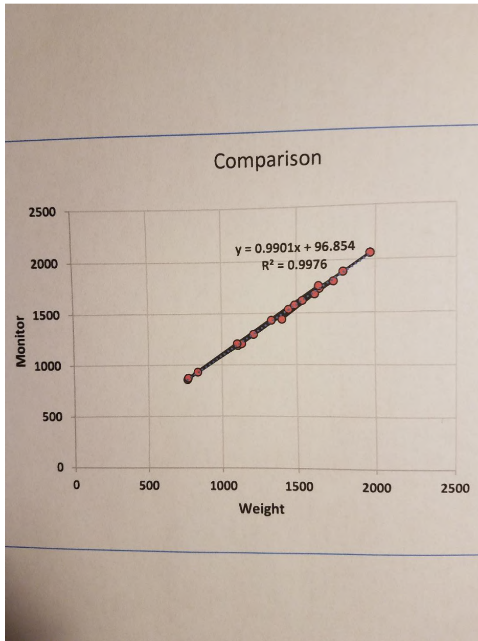
Photo 3. Screenshot of preharvest yield monitor calibration for certification, 2024.
