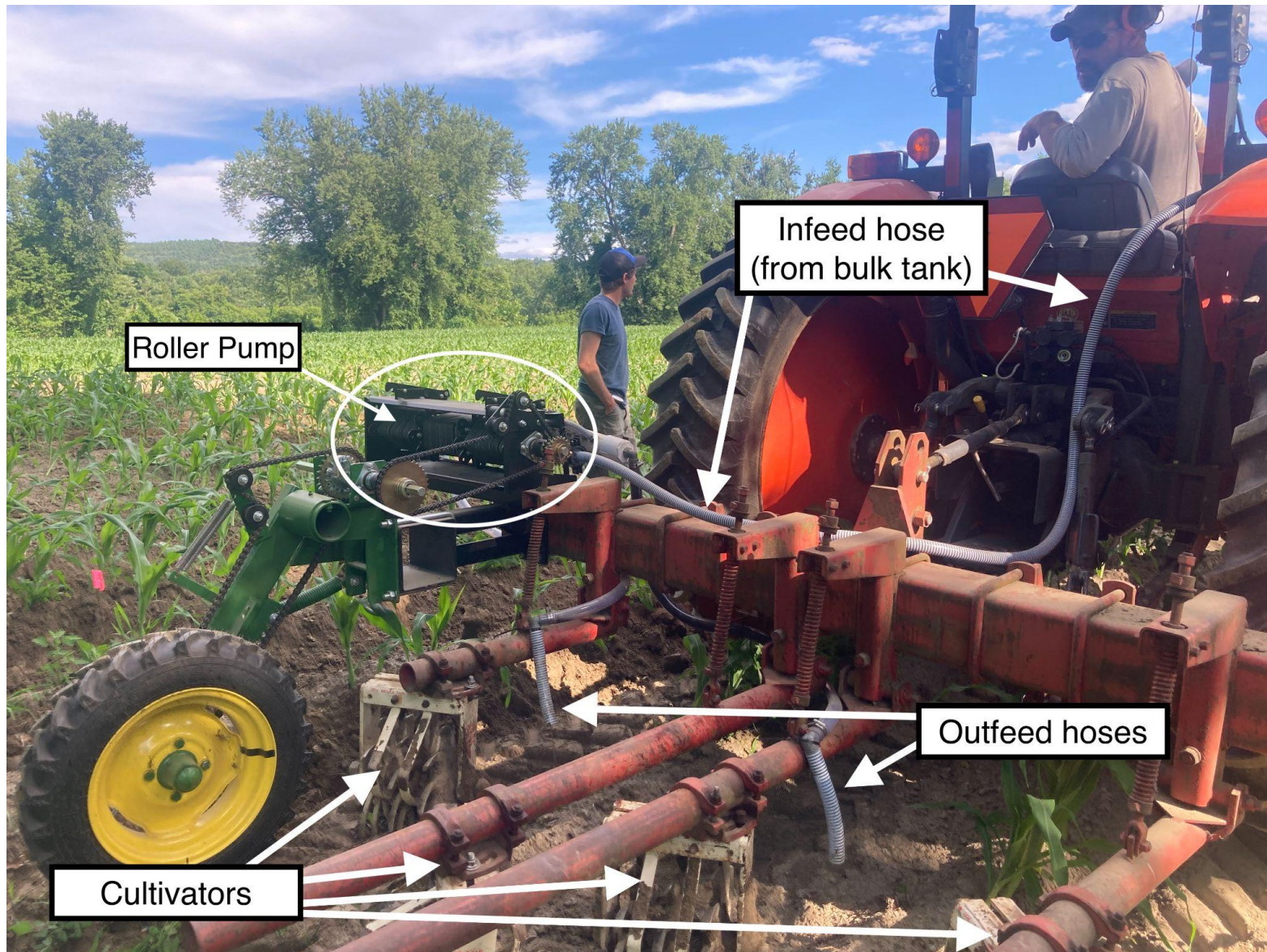
Photo 2: Infeed hose goes to roller pump and outfeed hoses attached to cultivator to direct fertilizer to corn rows.
