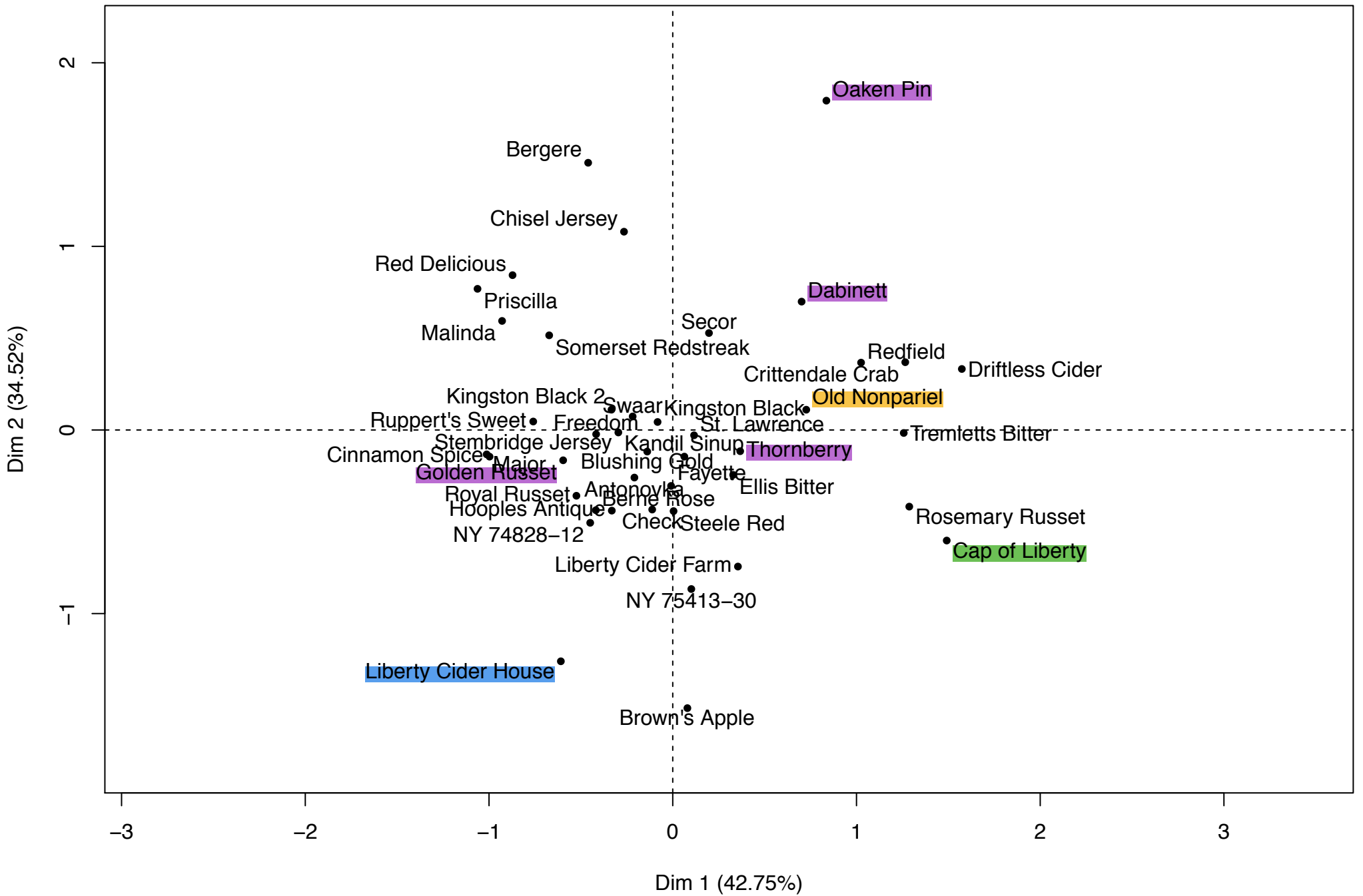
Individuals factor map (PCA)
