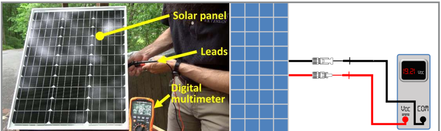
Figure 5. The open-circuit voltage ( V_{oc} ) of a 50 watt solar module is measured (left) by connecting the positive lead of a digital multimeter to the positive PV terminal, and the negative lead of the digital multimeter to the negative PV terminal (right). An open circuit voltage of 19.21 V was measured during less than full sun conditions.
