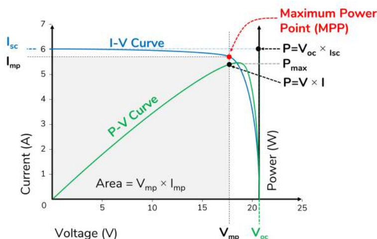
Figure 8. Characteristic current-voltage (I-V) and power-voltage (P-V) curves based on voltage and current measurements of a solar module at variable resistance loads. Power data was evaluated based on voltage and current values according to Watt’s Law ( P=I \times V ).
