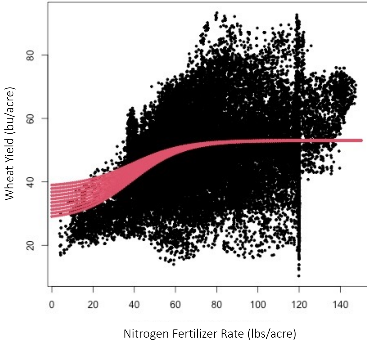
Grain Yield Response to Nitrogen Fertilizer Application on Farm 2
