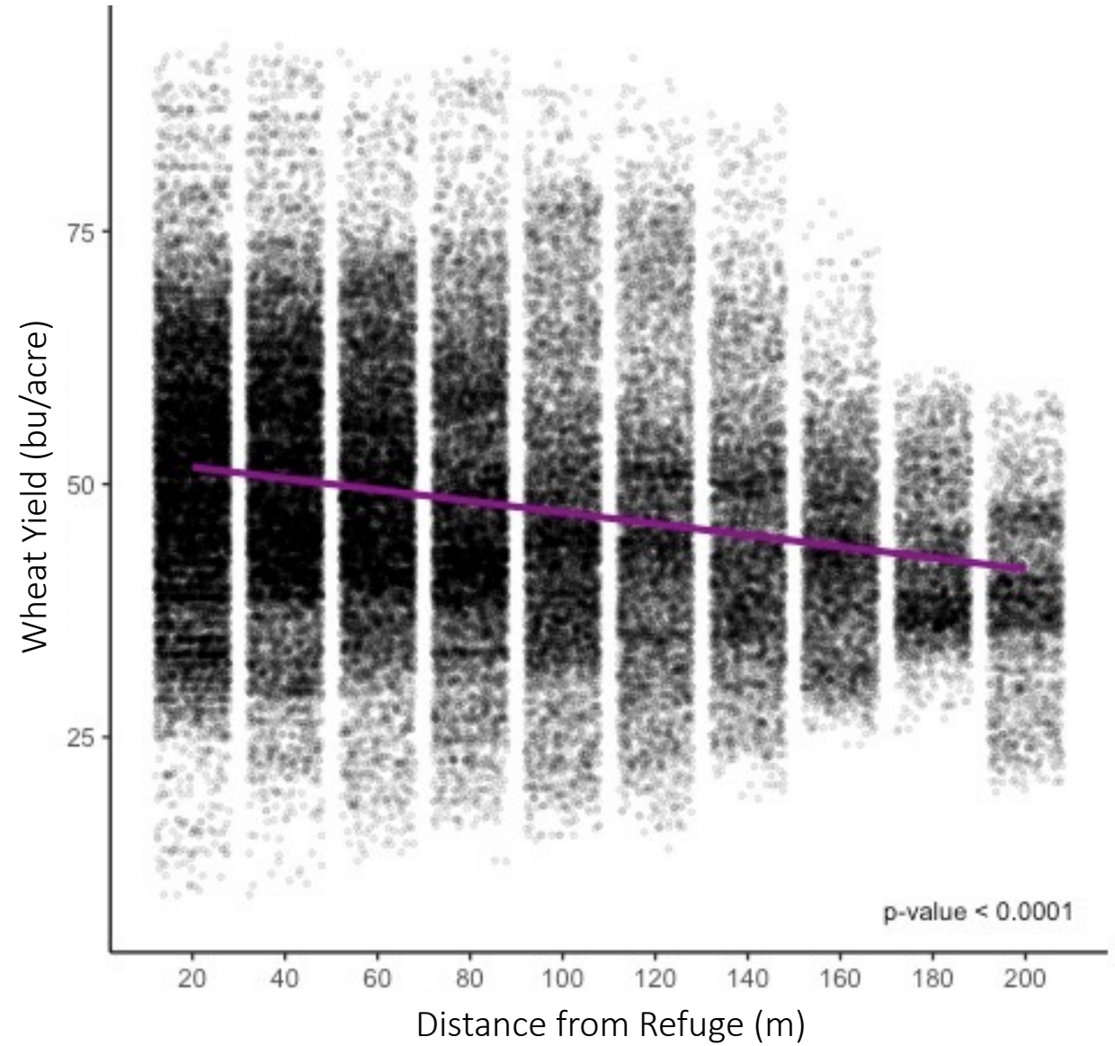
Grain Yield Response to Distance from Refuge on Farm 2
