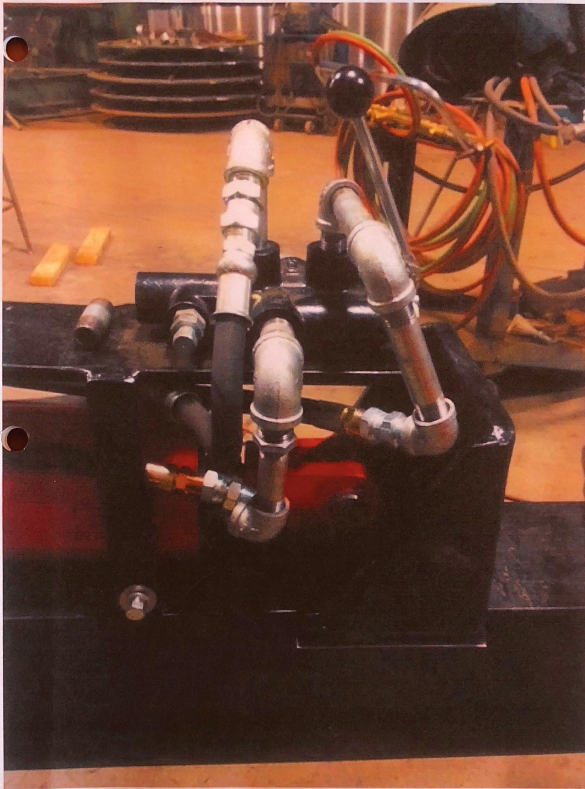
Hydraulic control unit - detent valve
