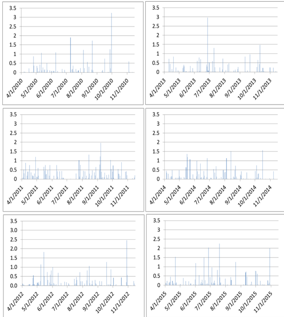
Figure 1: PSU NESARE dairy cropping systems daily growing season precipitation (in) (2010-2015).
