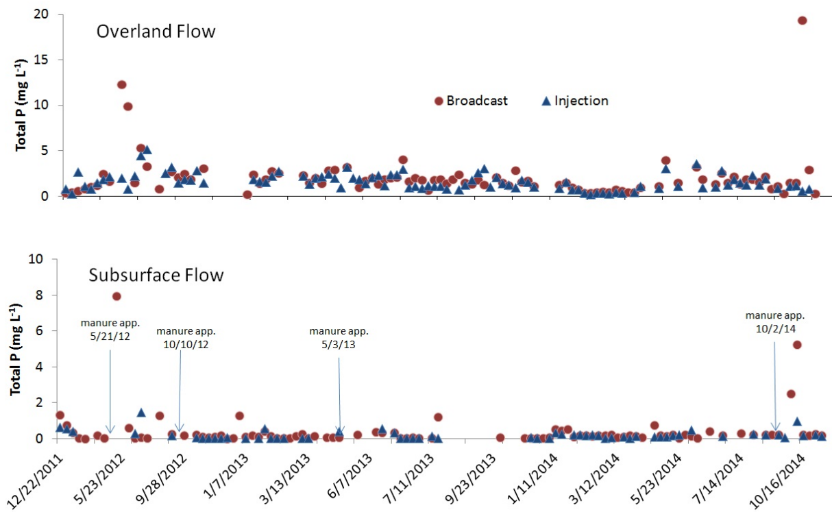
Figure 6: Total Phosphorus (P) concentration in overland and subsurface flow for storm events
