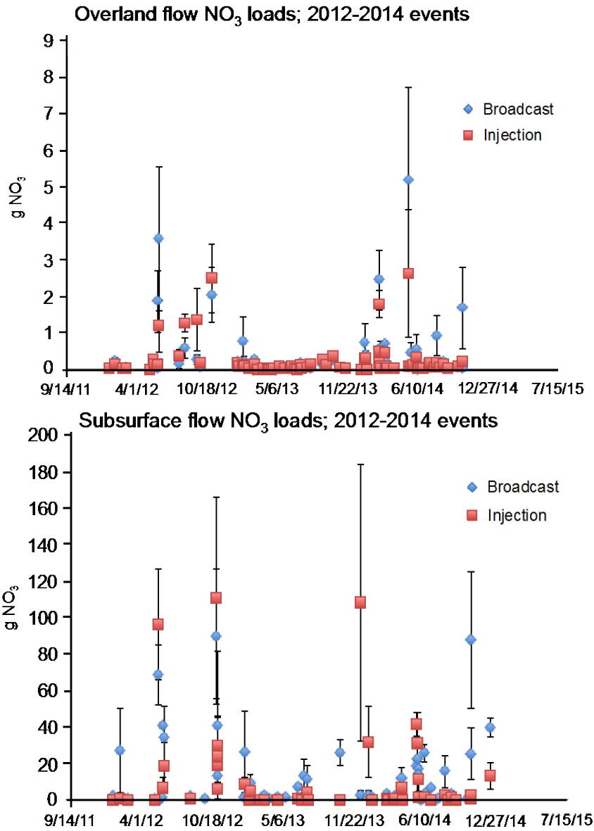
Figure 4: Overland and subsurface flow of nitrate loads as affected by broadcast manure and manure injection
