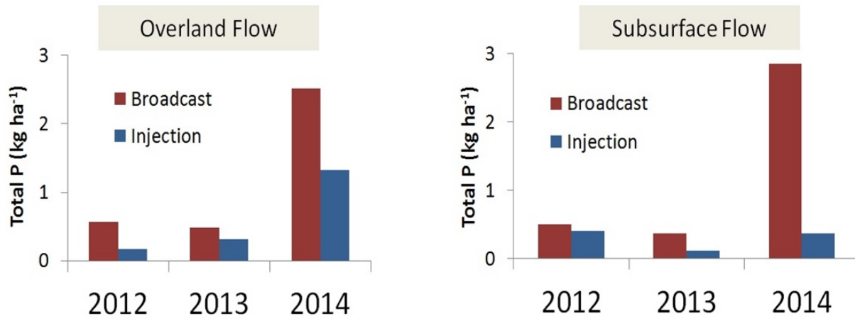
Figure 5: Average annual total phosphorus (P) yield for the lysimeter Plots.
