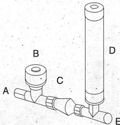
Figure 2. Key features of a ram pump. This pump works by having water move into the pump from point A through B and C. There is a rubber bladder in D that compresses as the water rushes in. As the bladder expands, a valve in B blocks the water from moving backwards, forcing it through area E. A cyclical pattern is established so that water flow to the water storage area is constant.
