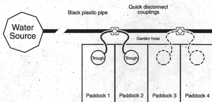
Figure 1. Setup of a quick-move watering system. Note that one coupling (on plastic pipe) can serve two or more paddocks.
