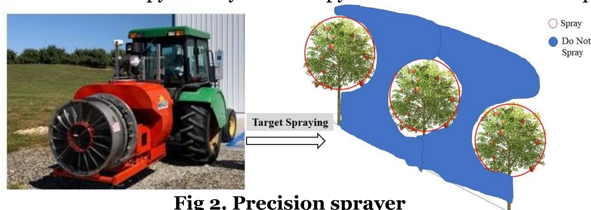
Fig 2. Precision sprayer
