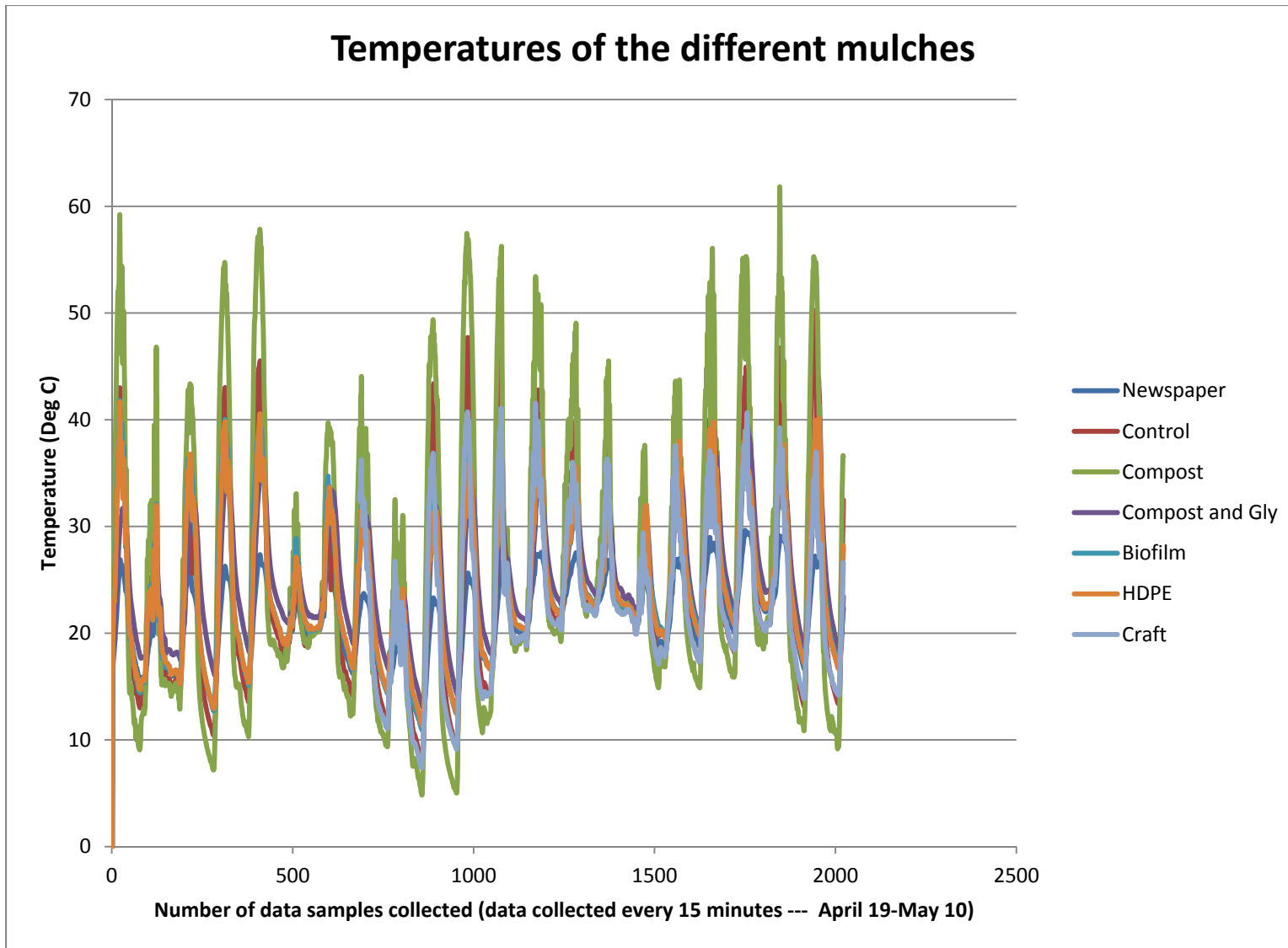
Figure 7. The temperatures of all mulches plotted on the same graph. Data was collected every 15 minutes.
