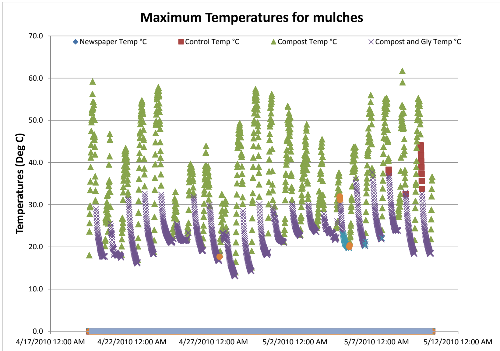
Figure 9. The maximum temperatures on a 15 minute base.
