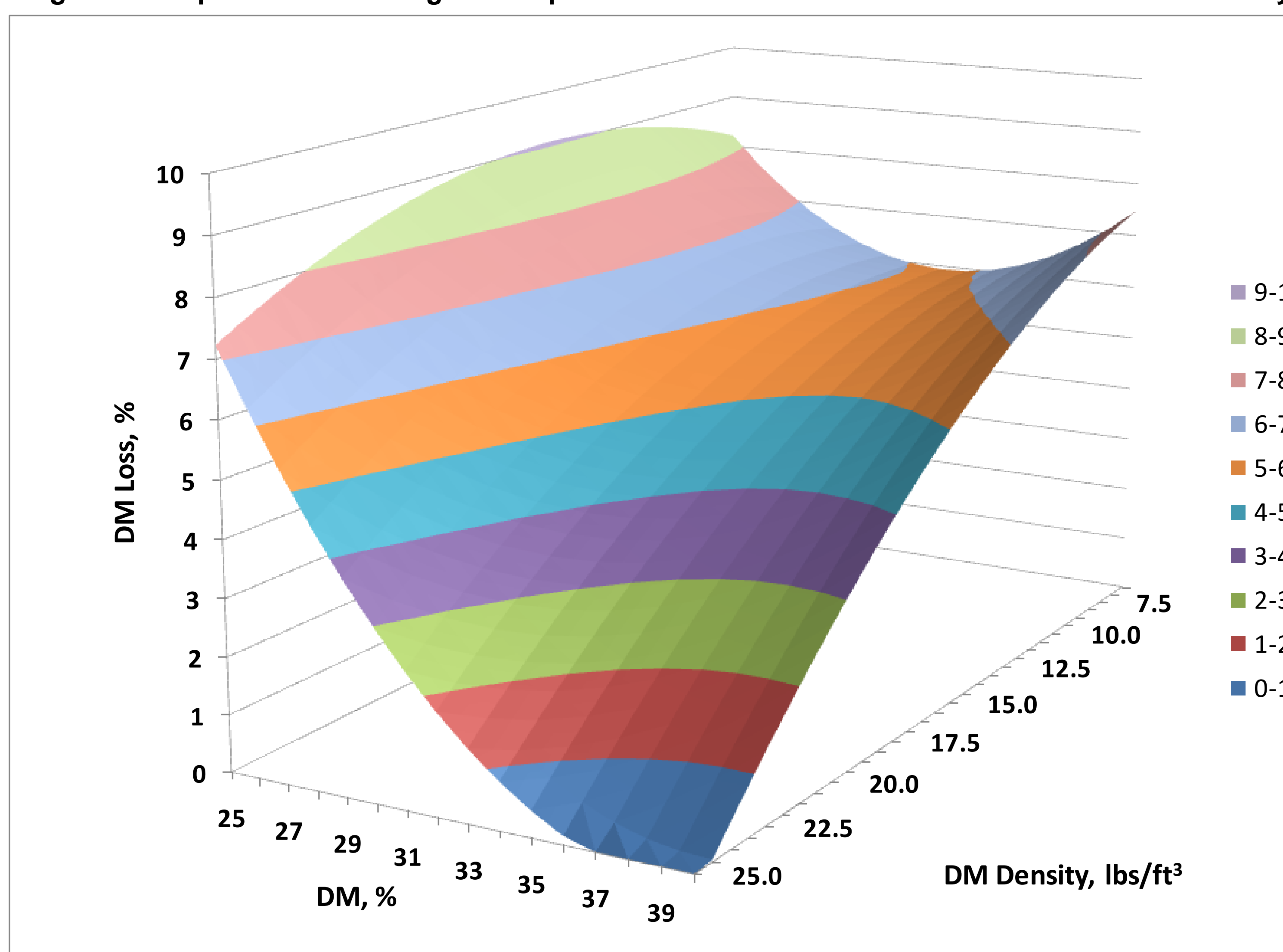
Figure 4. Response surface regression prediction of DM loss as related to DM % and DM density.
