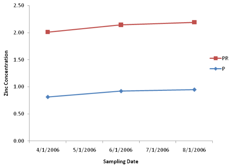
Figure 16: Changes in zinc concentration with sampling time between pinto bean monoculture and pinto bean-annual ryegrass intercrop treatments.
