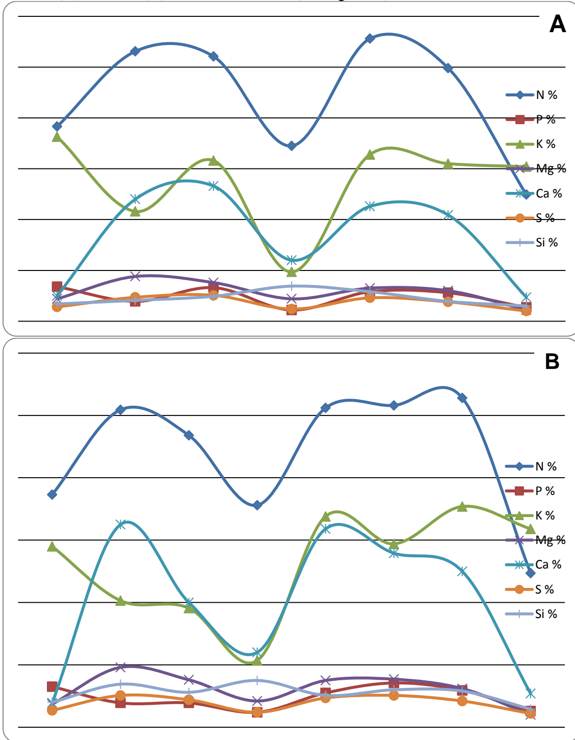
Figure 1. Elemental tissue analysis of field-grown cucumber ‘Straight Eight’ in Citra, FL without (A) and with (B) Si soil amendment (600 kg Si/ha)
