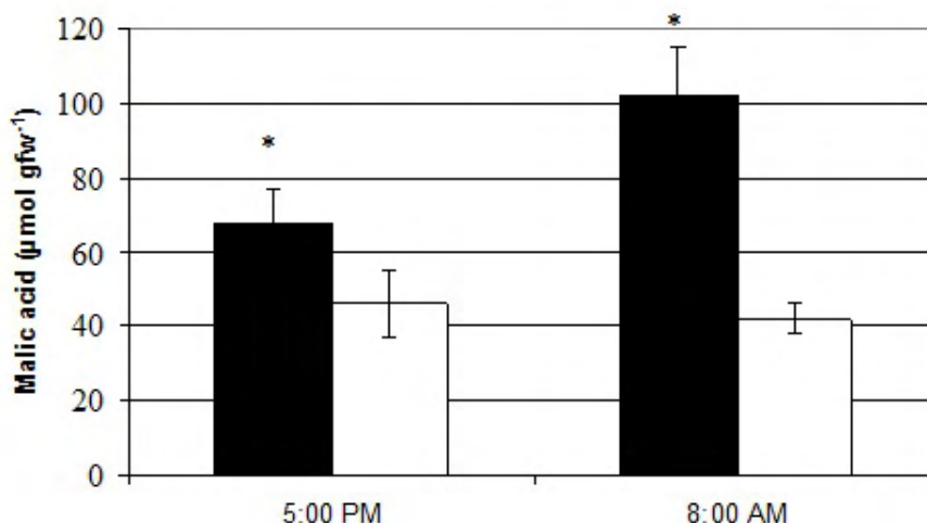
Figure 2. Nocturnal malic acid build-up in pineapple crown leaves from 5:00 p.m. to 8:00 a.m. after 7 days of post-transport treatment (n = 8 fruits). Diurnal light cycle at 10 °C (black bars); continuous dark at 10 °C (white bars). Statistically significant nocturnal malic acid build-up (*P<0.05) is indicated by *.
