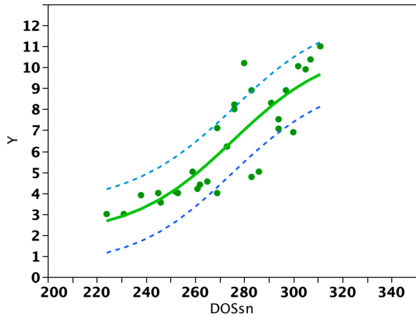
Figure 6. Progression of medusahead phenological stages as a function of days since the beginning of the season (1 Aug) for the twelve sites in the experiment.
