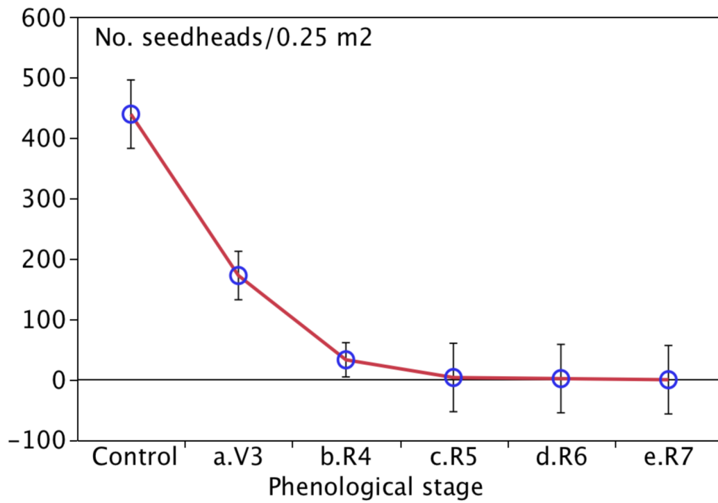
Figure 23. Effect of clipping at different phenological stages on total number of seedheads produced by goatgrass.
