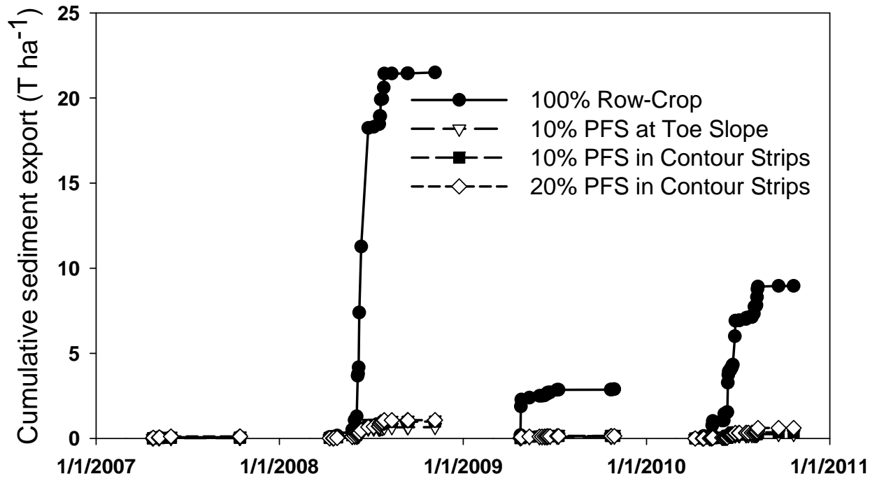
Figure 2: Sediment export in 2007, 2008, 2009, and 2010 (PFS – prairie filter strips)
