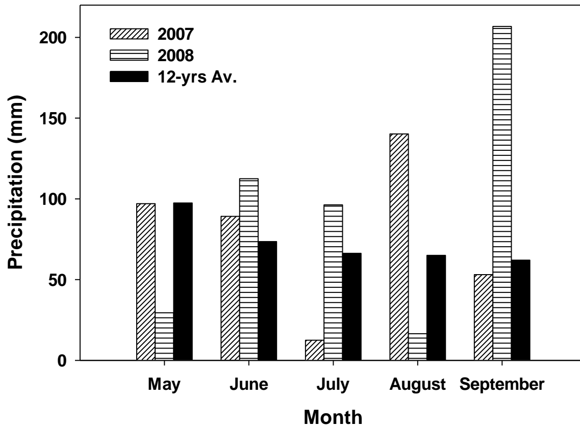
Figure 1 (A) Total monthly precipitation and during the 2007 and 2008 growing seasons compared with the 12-year monthly average at MSU’s Horticultural Farm, East Lansing, MI.
