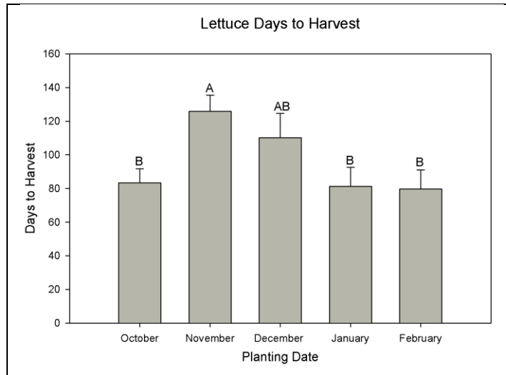
Figure 10. Average days to first harvest of lettuce by planting date. Differing uppercase letters signify statistical differences between planting dates at p \leq 0.05 according to least square means utilizing the Tukey adjustment.
