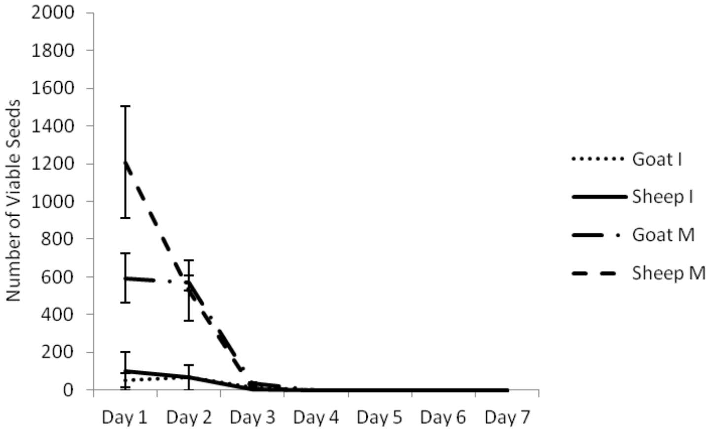
Figure 4. Mean number of viable sulfur cinquefoil seeds recovered per animal from the feces of sheep and goats over a 7-day period following oral gavage of 5,000 immature or mature seeds per animal. Error bars depict the standard error of the mean ( \alpha = 0.05 ).
