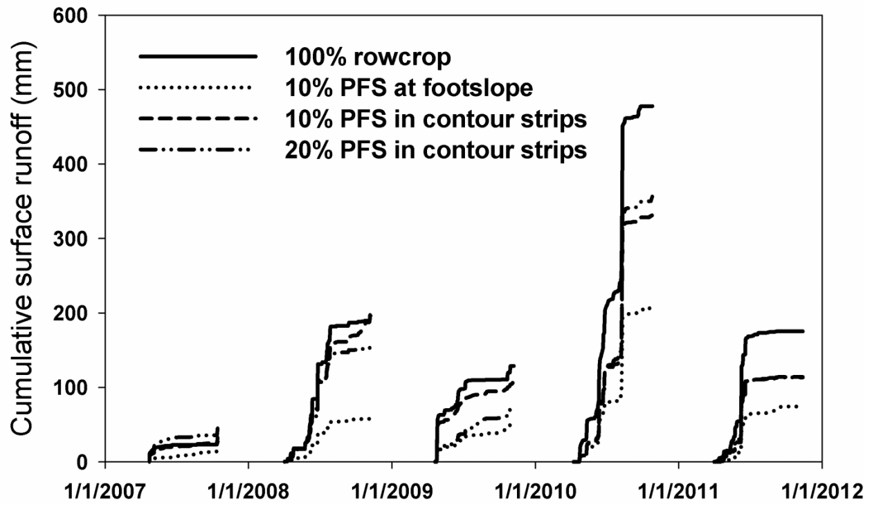
Figure 1: Surface runoff in 2007, 2008, 2009, 2010, and 2011 (PFS – prairie filter strips)
