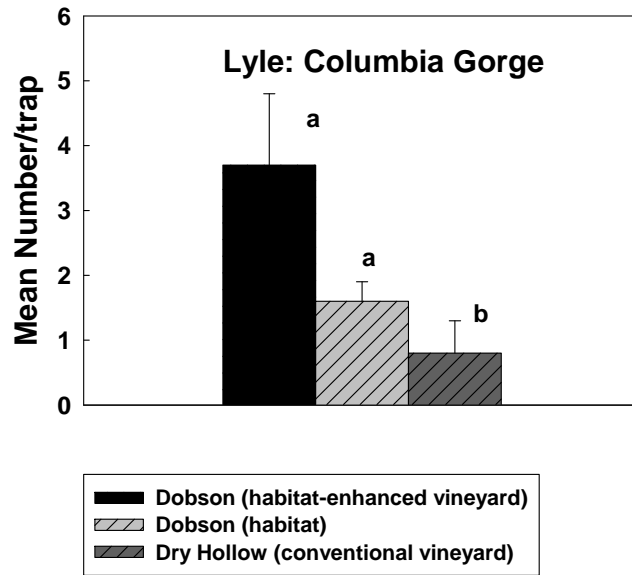
Figure 9. Abundance of beneficial beetles and bugs in a conventional (habitat-reduced) and a habitat-enhanced vineyard and adjacent habitat in the Columbia Gorge in 2012.
