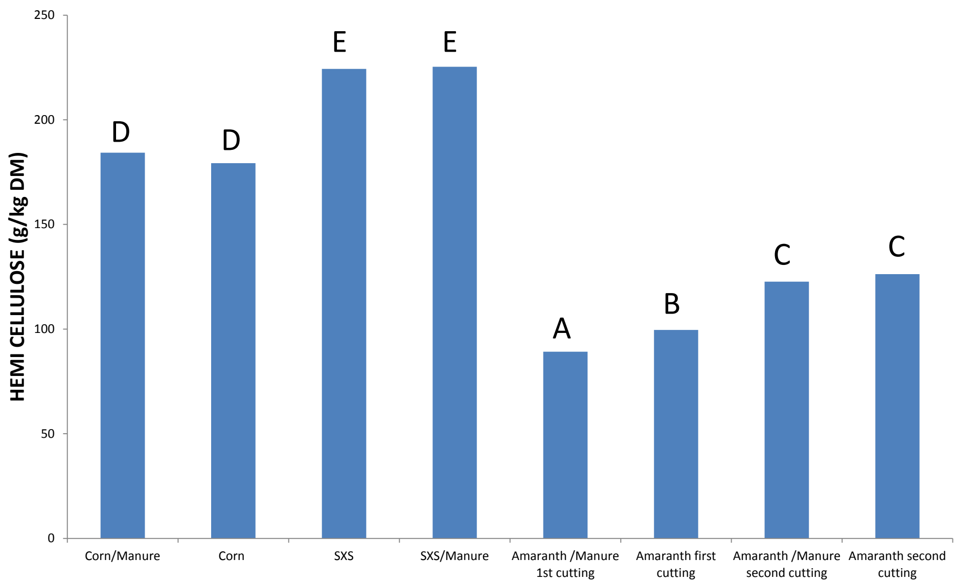
Figure 5. Hemi-cellulose content of treatments in 2011. Treatments are represented as either manure or no manure. BMR sorghum sudangrass is abbreviated as SXS. Treatments with different letters are significant at the \alpha -p-value=0.05 level
